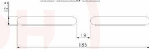
Vent Routing Detail
