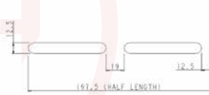
Vent Routing Detail
