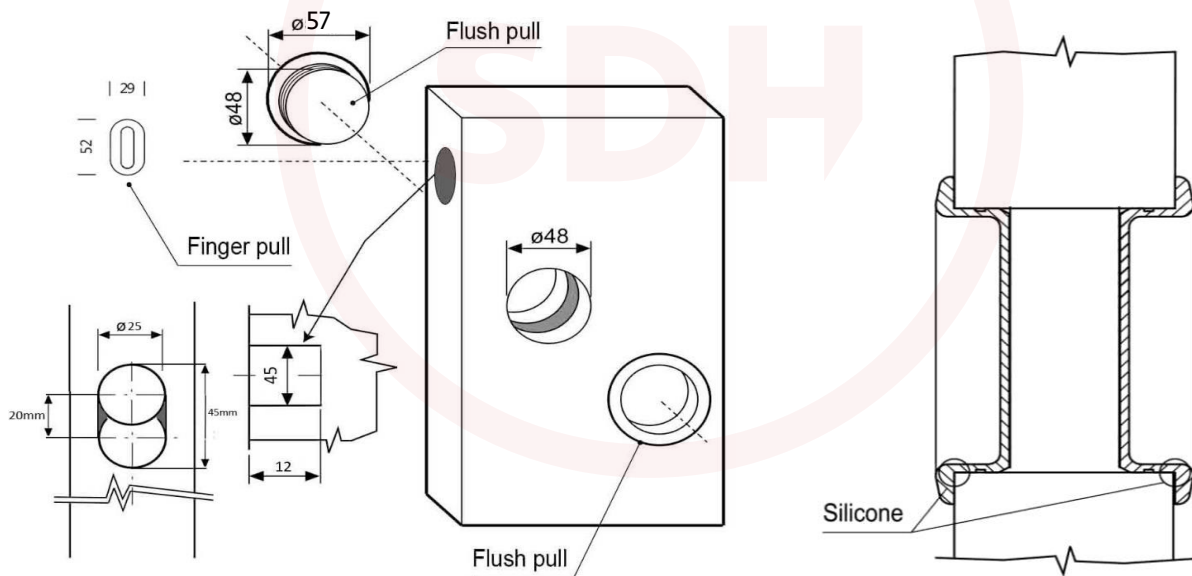
Diagram 1. Drilling dimensions
