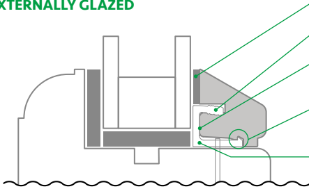
SECTION DRAWING FOR USE OF SD3 GLAZING BEAD
