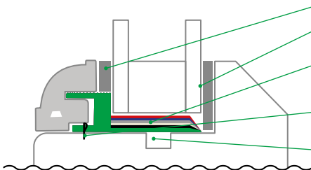
SECTION DRAWING FOR USE OF SD2 GLAZING BEAD
