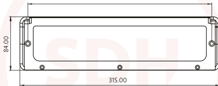
Routing Detail
